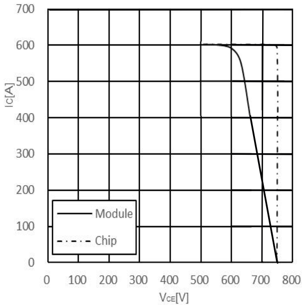
Reverse bias safe operating area IGBT, Inverter(RBSOA) IGBT 反向安全工作区, 逆变(RBSOA) I_c = f(V_{CE}), V_{CE} = +15V/-8V, R_{Goff} = 7.5\Omega, T_j = 150^\circ C
